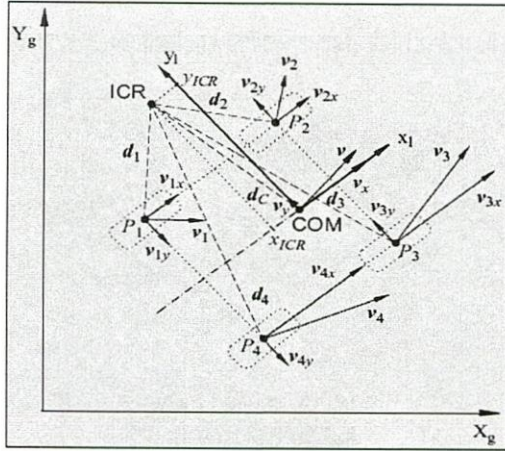
Fig. 5. Wheel velocities.
