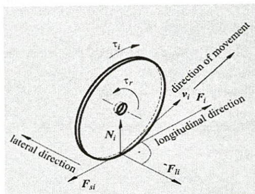
Fig. 6. The forces acting on one wheel.
