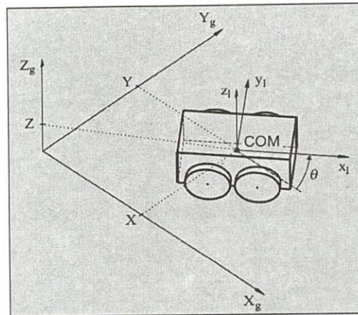
Fig. 2. The robot in the inertial frame
