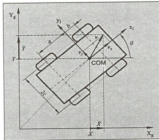
Fig. 3. Schematic of the skid steering robot.
