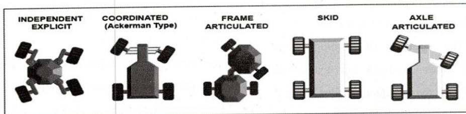
Fig. 1 Kinematics of major steering types
