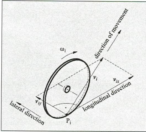
Fig. 4. Velocities of one wheel.
