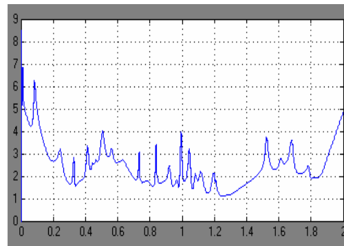
Fig 9. The demonstration of \|\varphi_2\|
