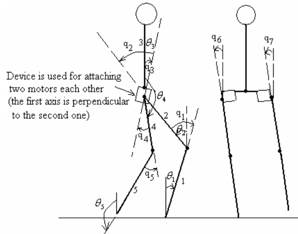
Fig1. The relative coordinates q_i
