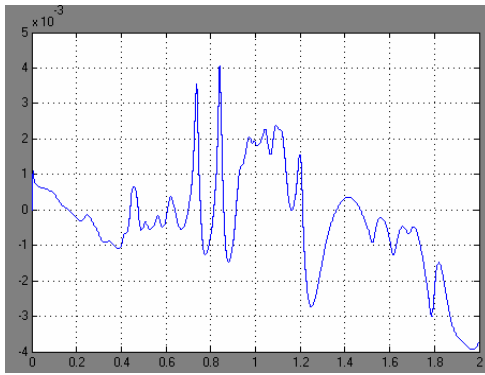
Fig 6. The error of the 5th joint (degree/s)
