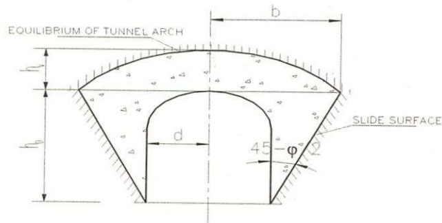
THE COLLAPSE DIAGRAM OF SOIL AROUND TUNNEL STRUCTURE
