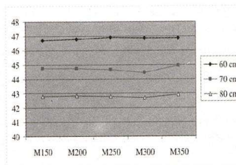
Figure 10. The relation of tunnel shell thickness, grade of concrete and angle u_0
