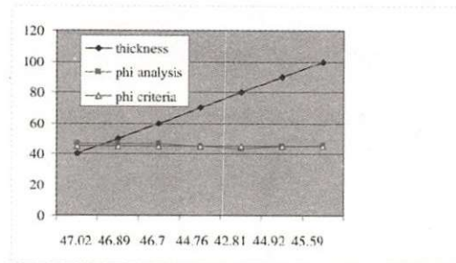
Figure 9. The relation of tunnel thickness and angle U_0
