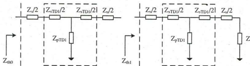
Fig A1. Equivalent Thevenin circuit
