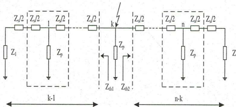
Fig 3. Equivalent circuit model
