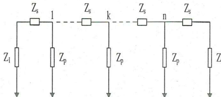
Fig 1. Equivalent circuit of grounding wire line
