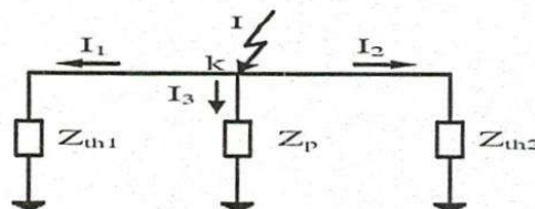
Fig 4. Equivalent Thevenin circuit
