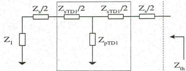
Fig 5. Equivalent circuit model to the left of the position that lightning strikes
