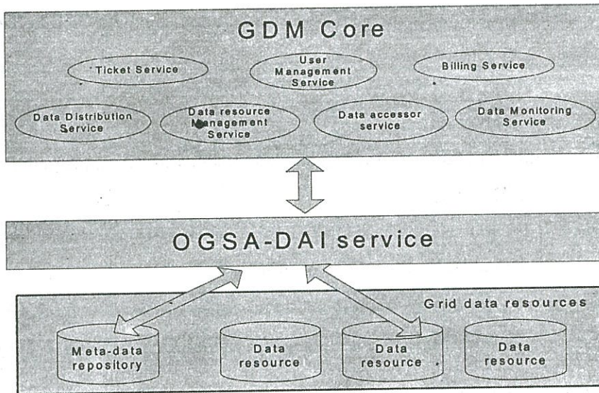
Figure 4. Implementation architecture of GDM framework.
