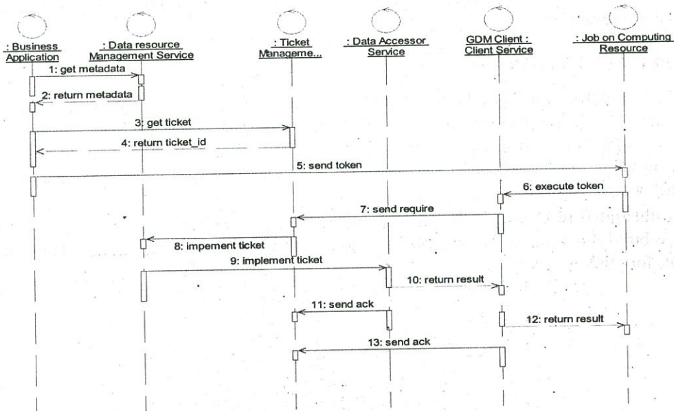
Figure 3. A typical interaction between an application and GDM.
