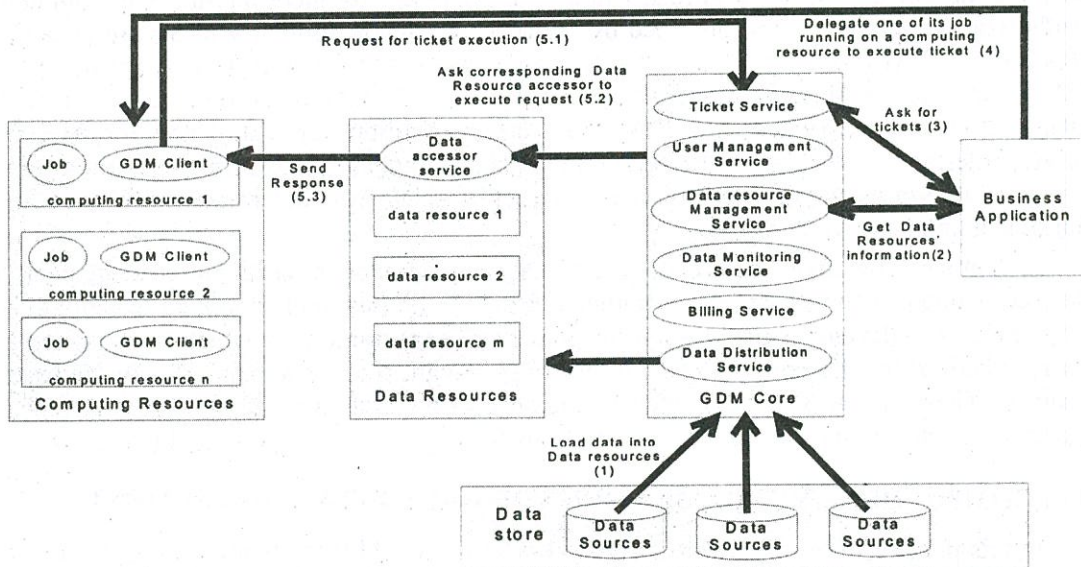
Figure 2. GDM framework architecture.
