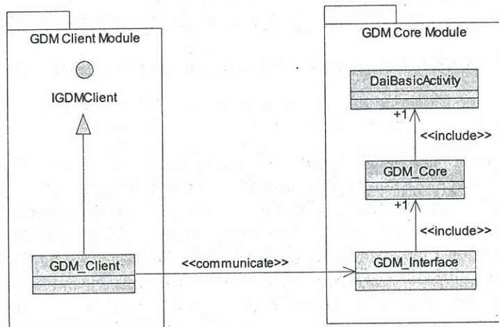
Figure 5. Class diagram of GDM implementation.
