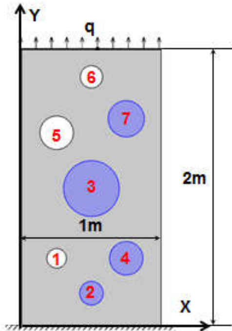
Figure 7. FGM plate with material variation in the x-direction with three circular holes and four circular inclusions We compare the finite element method (FEM) solution to that obtained by XFEM.
