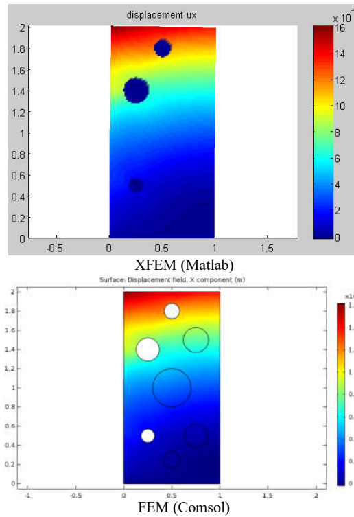
Figure 8. Comparison of displacement results u_x between XFEM and FEM
