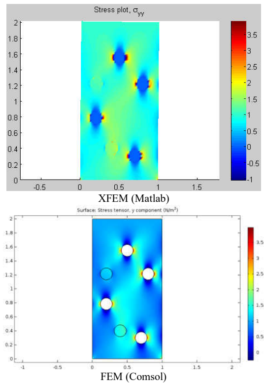
Figure 6. Comparison of stress results \sigma_{yy} between XFEM and FEM
