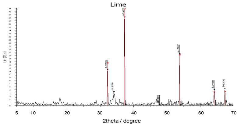
Figure 3. XRD pattern of commercialized CaO.
