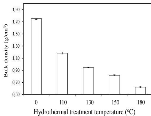
Figure 6. Bulk density of sample before and after hydrothermal treatment at different temperatures.
