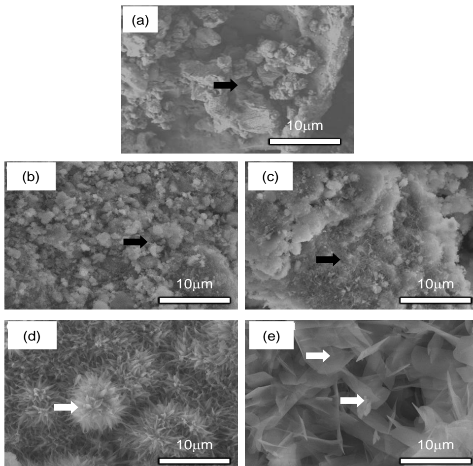
Figure 5. SEM images of sample before and after hydrothermal treatment at different temperature: (a) before; (b) 110°C; (c) 130°C; (d) 150°C and (e) 180°C.
