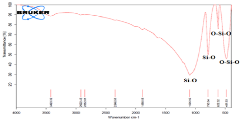
Figure 2. FTIR spectrum of RHA
