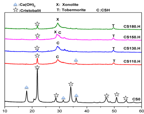
Figure 4. XRD patterns of compacted disk before and after hydrothermal treatment at various temperature: (a) before; (b) 110°C; (c) 130°C; (d) 150°C and (e) 180°C
