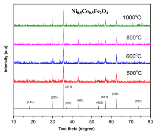
Figure 1. XRD patterns of Co_{1-x}Ni_xFe_2O_4 (with x=0.5 ) calcined at 500^\circ C , 600^\circ C , 800^\circ C and 1000^\circ C for 1 hour
