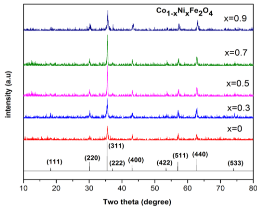
Figure 2. XRD patterns of \text{Co}_{1-x}\text{Ni}_x\text{Fe}_2\text{O}_4 which were calcined at 600°C for 1 hour.
