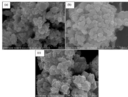
Figure 3. The SEM images of the \text{Co}_{1-x}\text{Ni}_x\text{Fe}_2\text{O}_4 powder; (a) x=0 ; (b) x=0.5 ; (c) x=0.9
