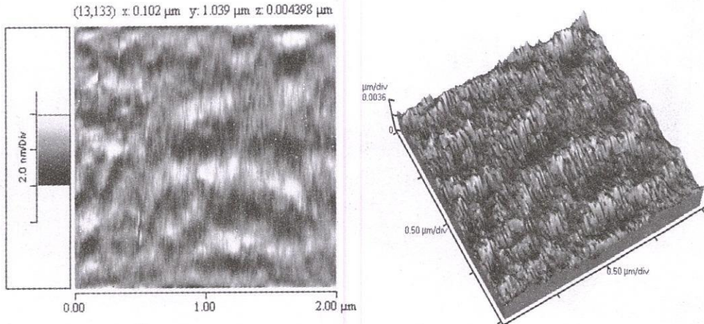
Hình 1c. \text{TiO}_2\text{-SiO}_2 (50 % \text{SiO}_2 ) : Rms Rough: 0.4431 nm;
