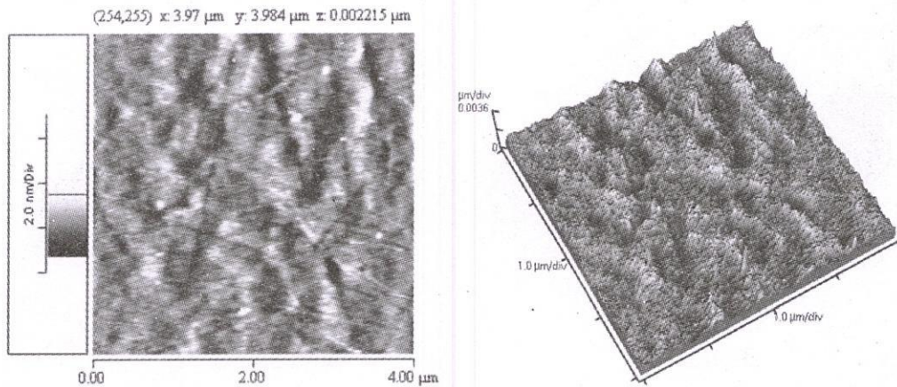
Hình 1d. \text{SiO}_2 (100 % \text{SiO}_2 ) : Rms Rough: 0.3286 nm;
