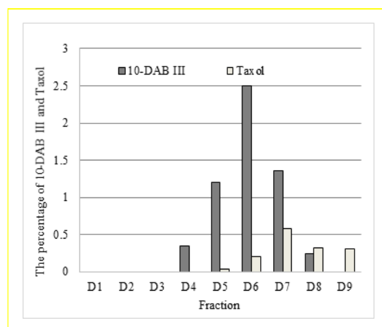
Figure 10. The percentage of 10-DAB III and Taxol after SPE using diaion column
